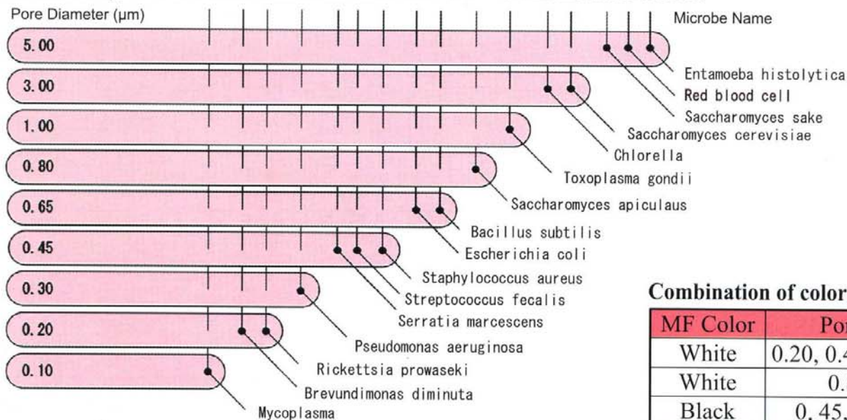
Relationship of Pore Size and Microbe Retention to Membrane Filters
